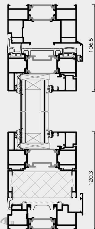
Vertical Section
