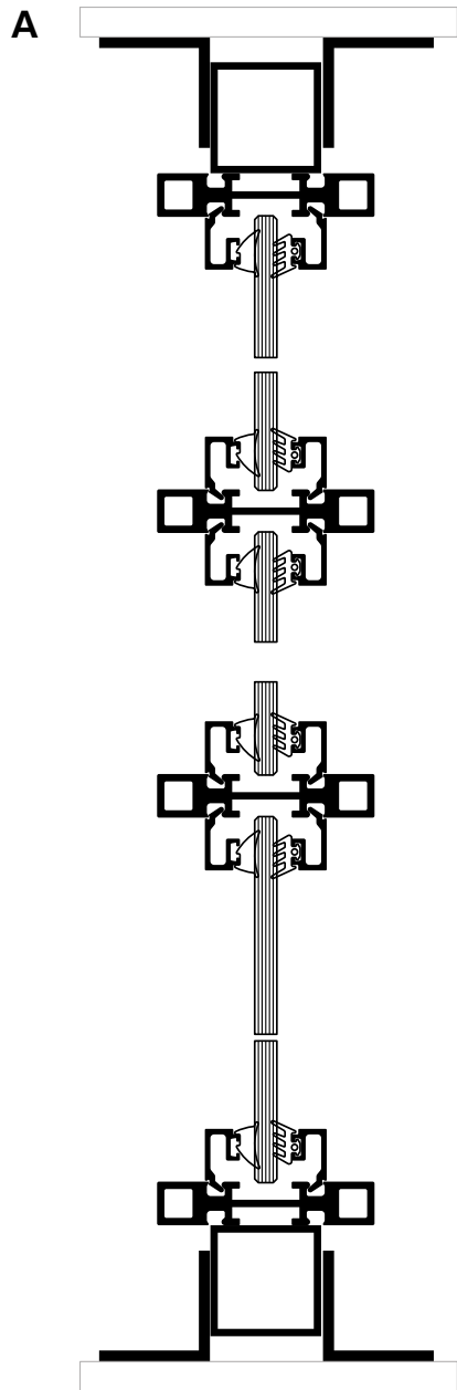
Vertical section of triple
