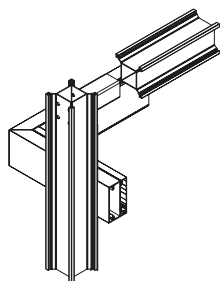
Mullion and transoms connection
