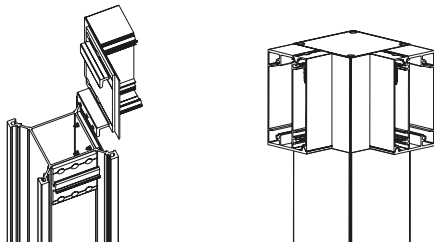
Mullion and transom connection
