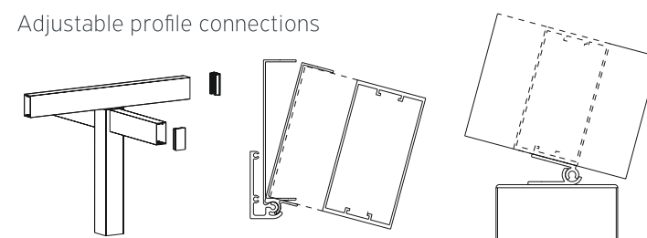
Adjustable profile connections
