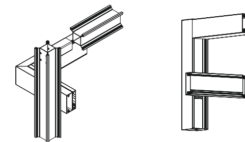
Mullion and transoms connection
